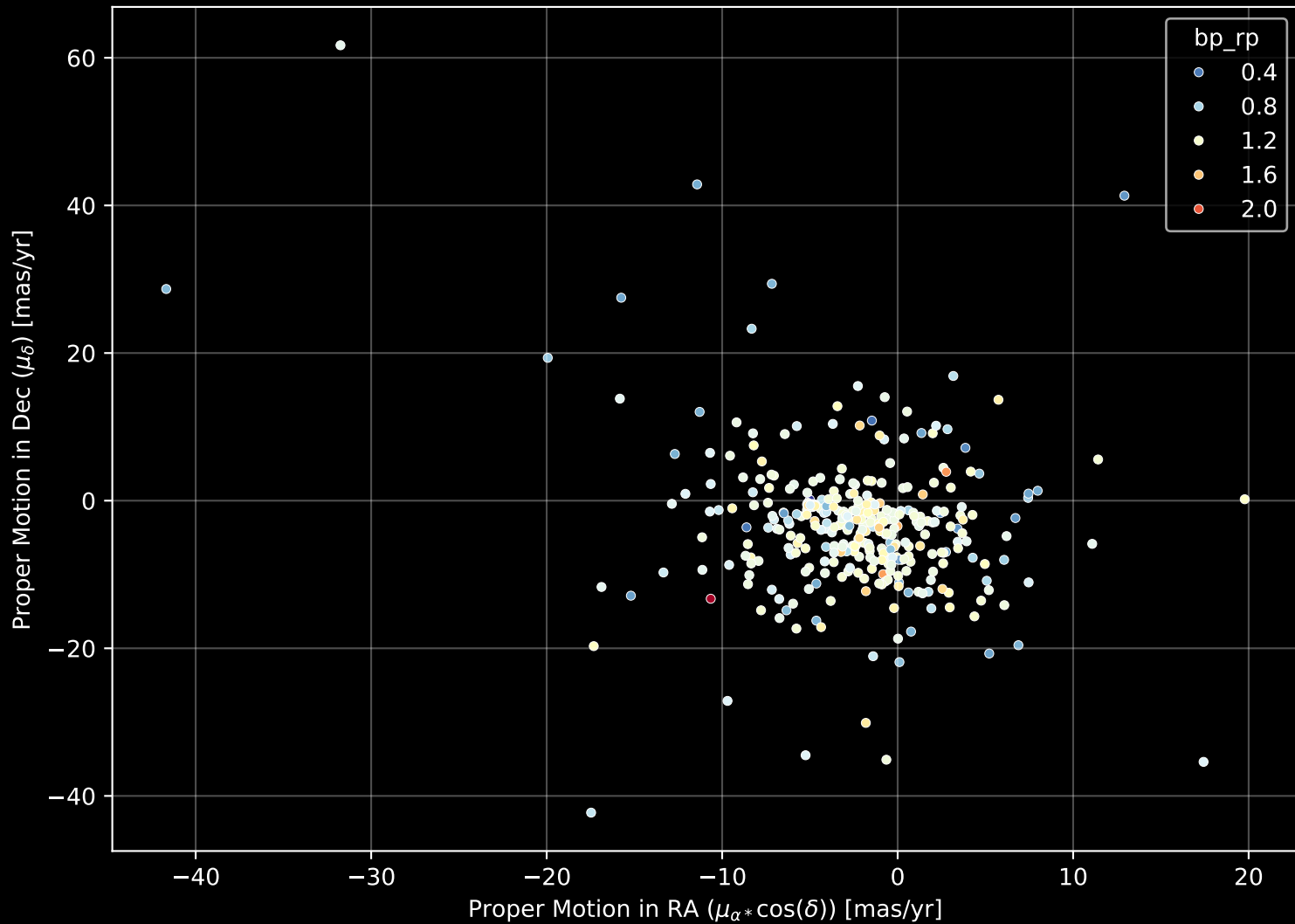
APOGEE DR17 Field: [M92] Proper Motion Diagram (n= 354)
