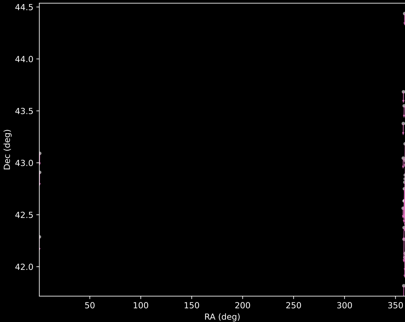
APOGEE DR17 Cluster 12 Proper Motion Vectors (n=23)
