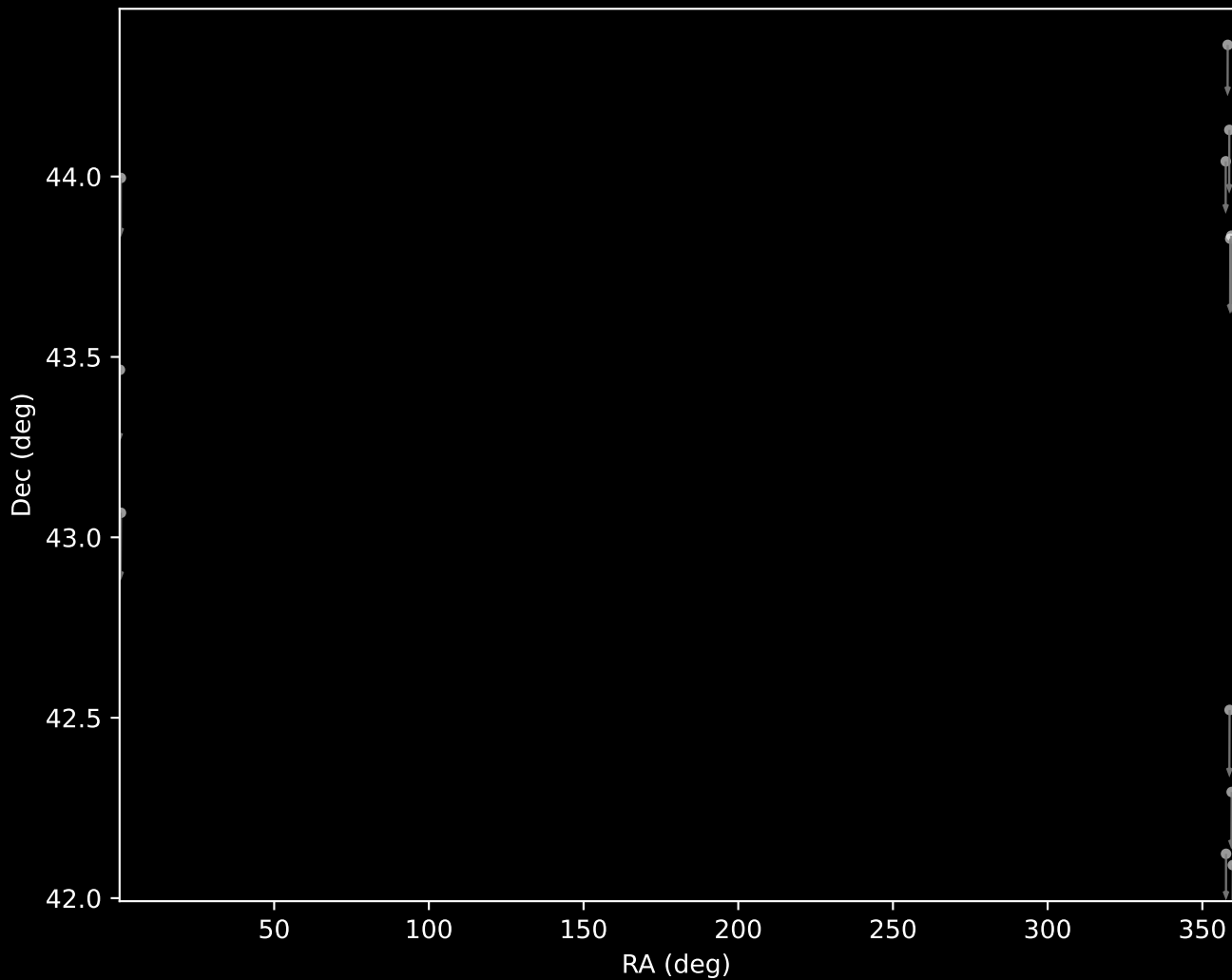
APOGEE DR17 Cluster 14 Proper Motion Vectors (n=12)
