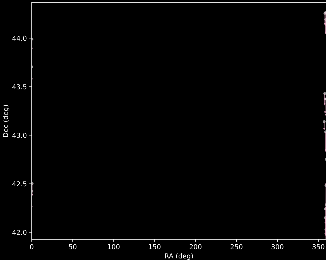
APOGEE DR17 Cluster 13 Proper Motion Vectors (n=18)
