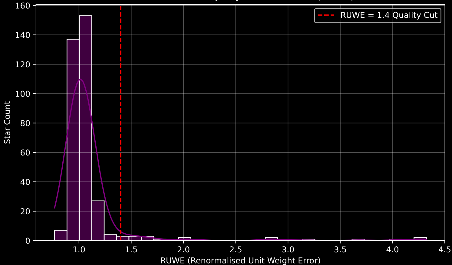
GAPOGEE DR17 Field [M92] RUWE Distribution (n= 347)
