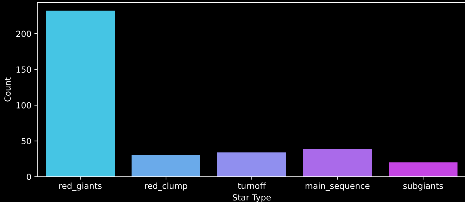
APOGEE DR17 Field: [M92] Count plot of Star Type
