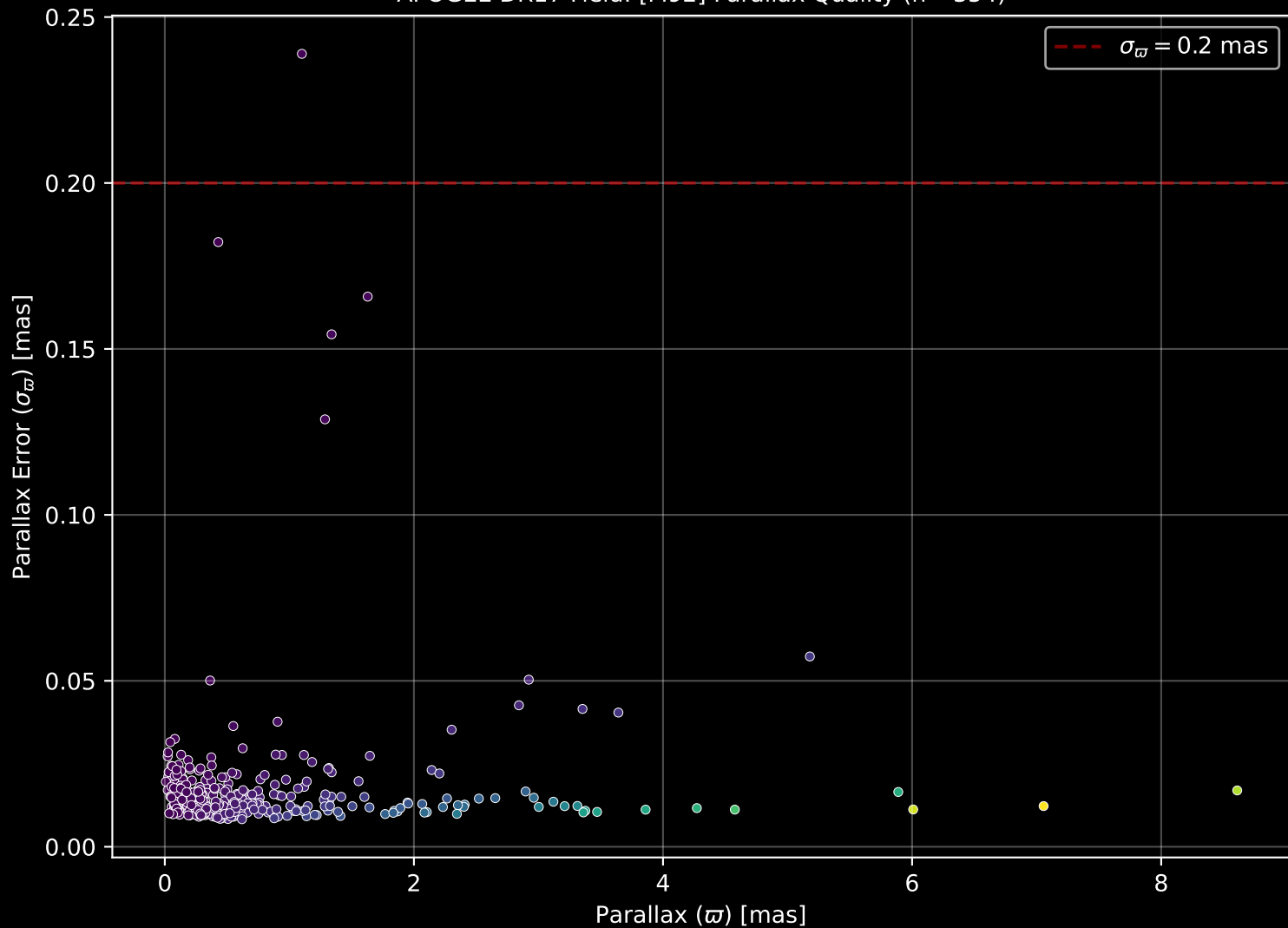
APOGEE DR17 Field: [M92] Parallax Quality (n= 354)
