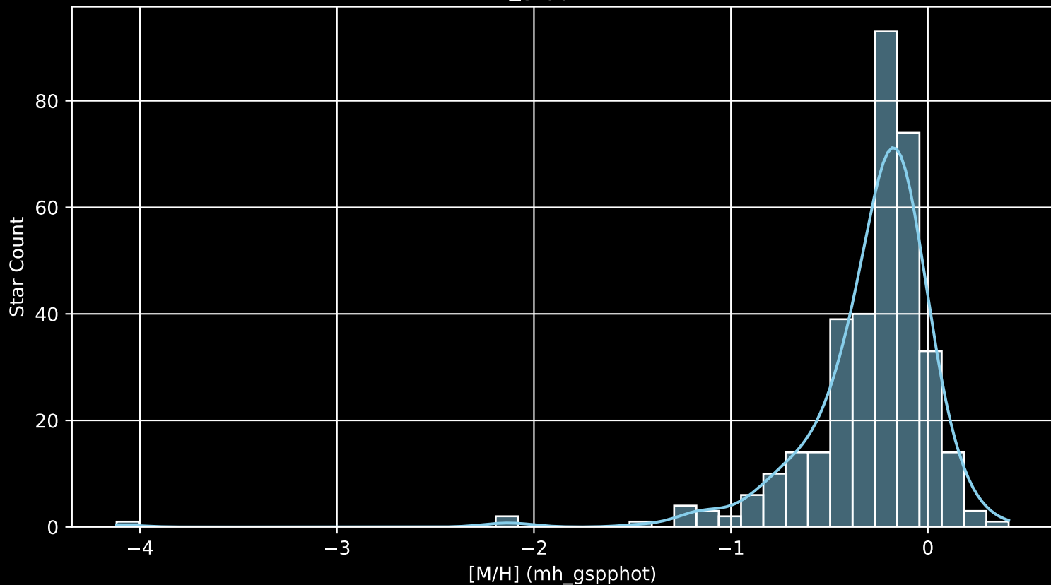
APOGEE DR17 Field: [M92 [M/H] (mh_gspphot) (n= 354)
