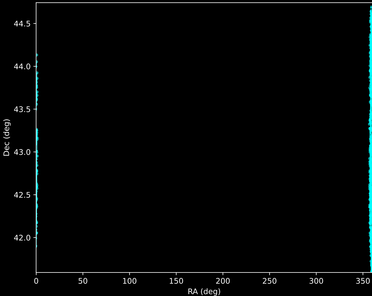
APOGEE DR17 Noise Stream Proper Motion Vectors (n=197)
